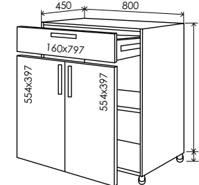
27 Низ 820*800 27/1 27/4 27/6
