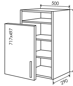
30 Верх 920*500 30/1
