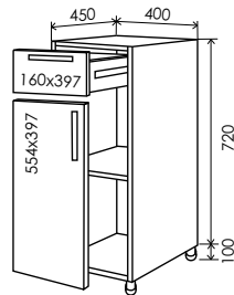
25 Низ 820*400 25/1 25/4 25/6
