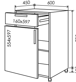
26 Низ 820*600 26/1 26/4 26/6
