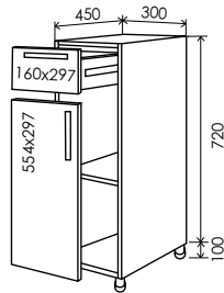
24 Низ 820*300 24/1 24/4 24/6
