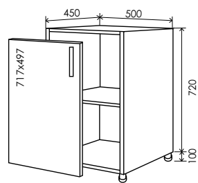
8 Низ 820*500 8/1
