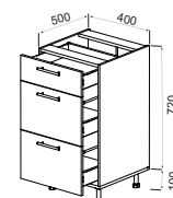
Низ 3Ш 400_500_720 (D403S) H-720mm., W-400mm.
